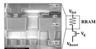
Fig. 1. (Left) SEM cross section of an integrated TiN/HfO 2 /Ti/TiN cell between M4 and M5. (Right) Schematic view of the 1T-1R cell
